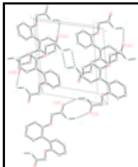
Fig. 2. Packing diagram of (I) with hydrogen bonds viewed along the b axis. Symmetry codes for A through D are: 1 - x, 1 - y, 1 - z ; x, 1 + y, z ; 1 - x, -y, 1 - z ; and 1 - x, 1 - y, 2 - z , respectively.
