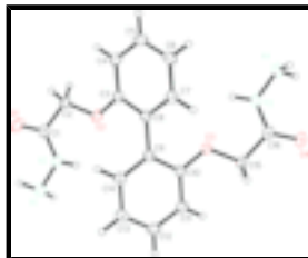
Fig. 1. Molecular structure of the the title compound showing 50% probability displacement ellipsoids with arbitrary shperes for H atoms.
